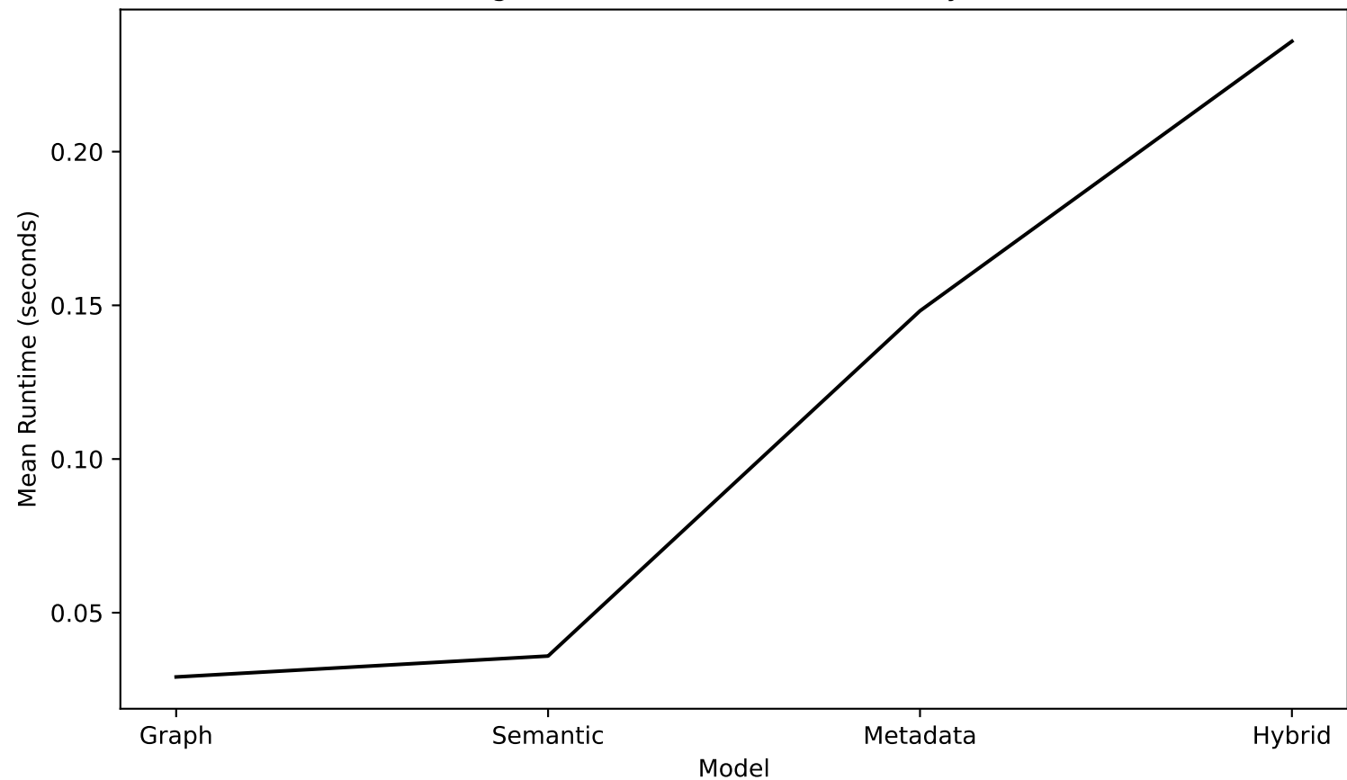
Average Recommendation Runtime by Model
